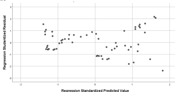
Gambar 3. Scatterplot
